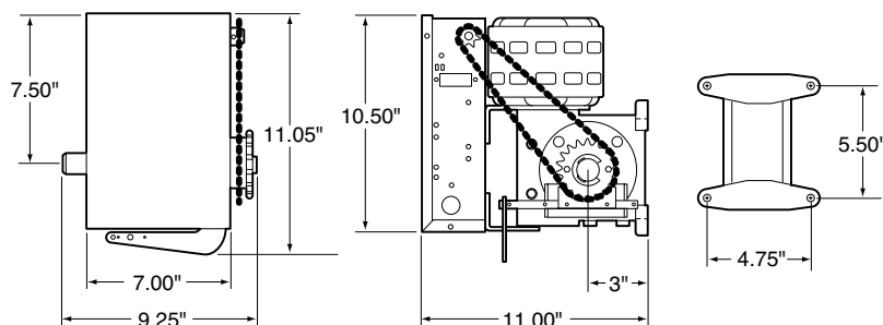
MOUNTING DIMENSIONS
